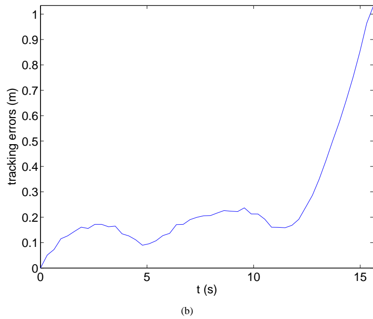
Figure 8: Experimental results without using the trajectory tracking module
