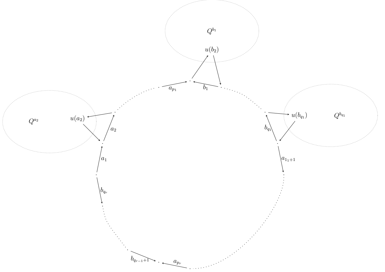
FIGURE 6.1. Shape of a quiver in \mathcal{M}_{p,q}^{\tilde{A}} .
