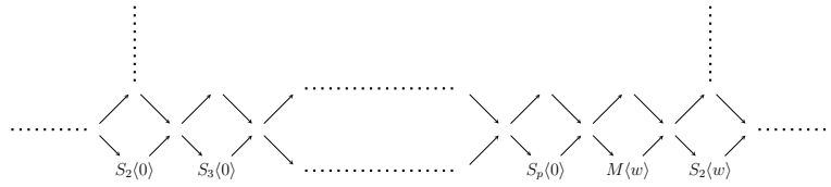
FIGURE 5.3. Shape of the connected component \mathcal{R}_0^p .
