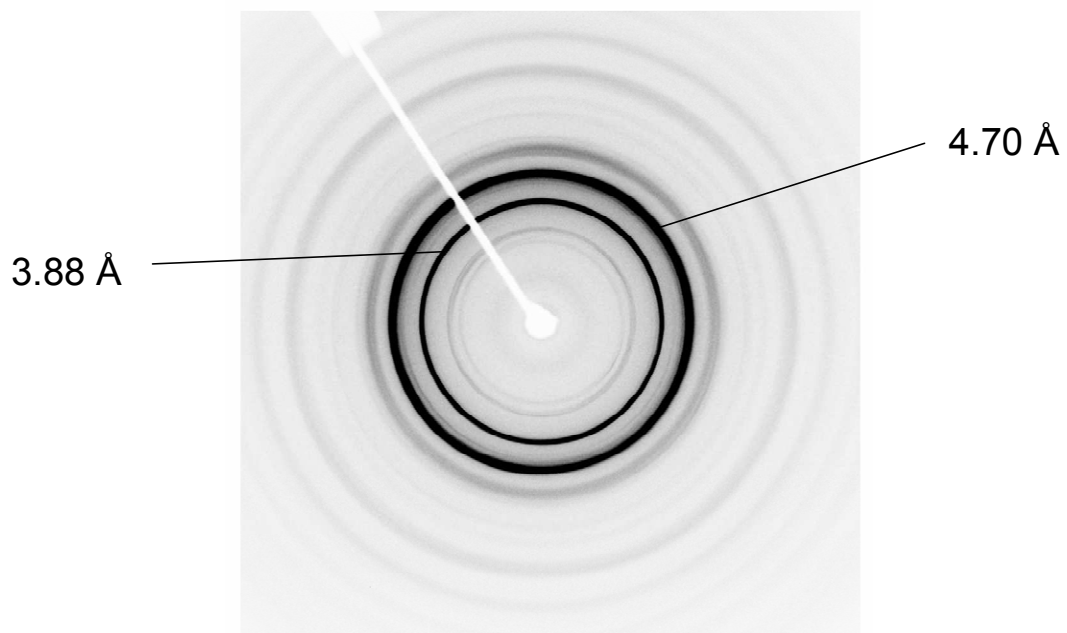
Figure 10. X-ray fibre diffraction pattern from a dried stalk of FFFF-PEG.
