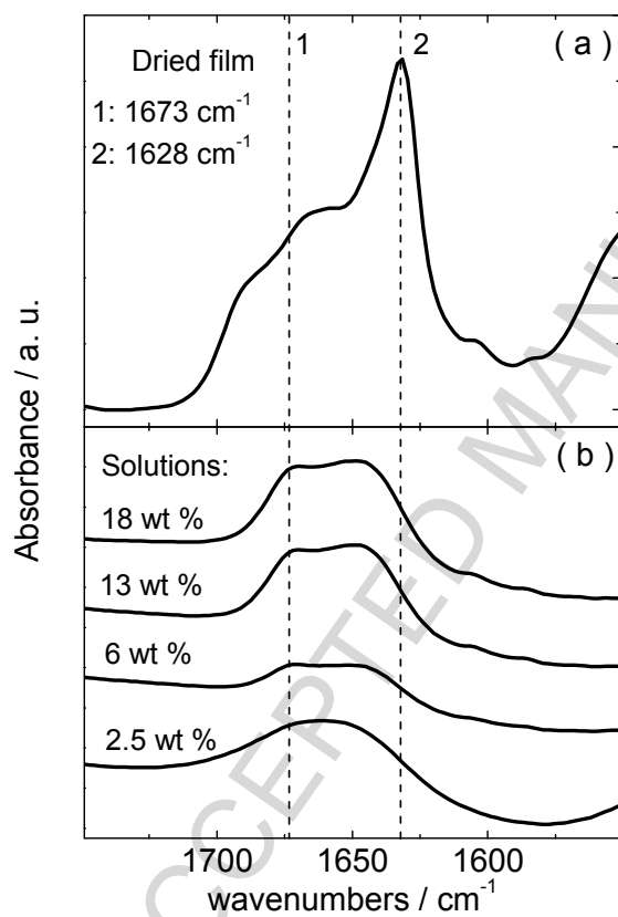
Figure 4. FTIR spectra of the amide I region of (a) a dried film of FFFF-PEG solution and (b) FFFF-PEG \text{D}_2\text{O} solutions containing 2.5, 6, 13, 18 wt% peptide. The peak positions 1 ( 1673 \text{ cm}^{-1} ) and 2 ( 1628 \text{ cm}^{-1} ) are associated with secondary structure in the dried film.
