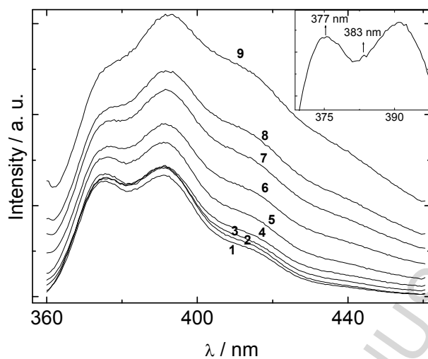
Figure 5. Fluorescence emission spectra for samples containing 3.6 \times 10^{-6} wt % pyrene and (1) 0, (2) 6.4 \times 10^{-3} , (3) 2.4 \times 10^{-2} , (4) 4.3 \times 10^{-2} , (5) 6.3 \times 10^{-2} , (6) 0.14, (7) 0.2, (8) 0.27 and (9) 0.4 wt % FFFF-PEG. The excitation wavelength was 339 nm. The inset shows spectrum 1 (pyrene only) on an enlarged scale.
