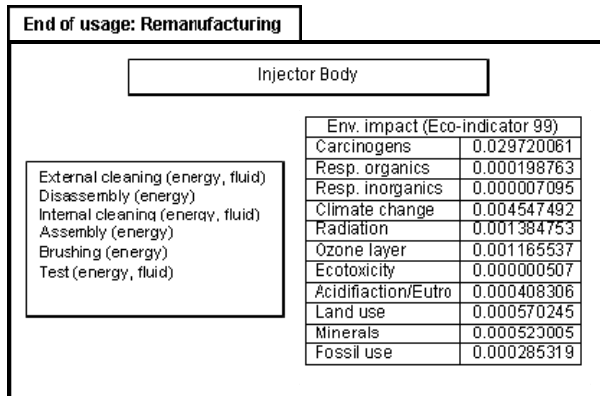
Figure 5: The remanufacturing life cycle brick for the body
