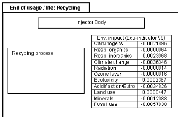
Figure 6: The recycling life cycle brick for the body
