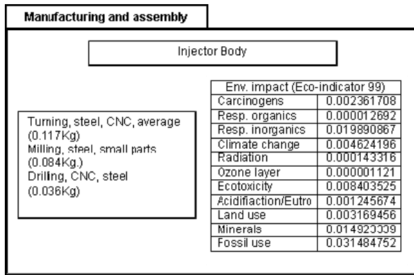
Figure 4: The manufacturing life cycle brick for the body Some components have different disposal scenario (figure 5, figure 6). So, different calculations of the environmental impact were realised. For the remanufacturing case, the processes were detailed, because they do not exist in the current databases. For the recycling, data from Simapro databases were used.
