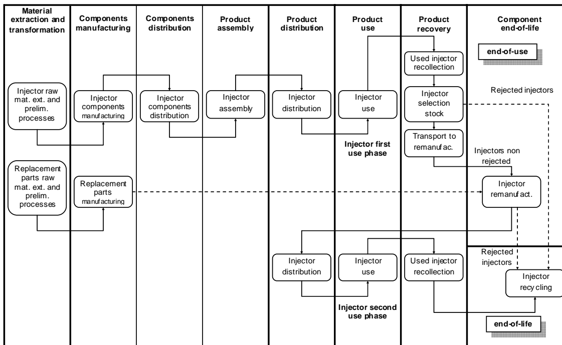
Figure 3: Injector diesel life cycle
