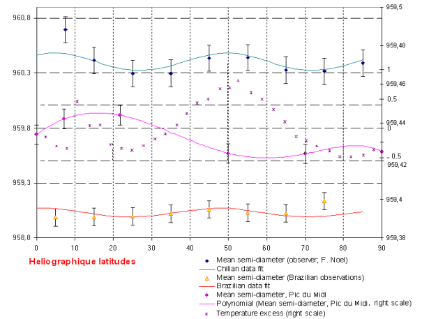
Figure 2: Comparison of the deviation to the mean solar radius obtained by means of the astrolabes, in Chili and Brazil (left scale). The deduced values of oblateness are not consistent with modern measurements. The data obtained at the Pic du Midi observatory (France) plotted versus the heliographic latitude is also shown (right scale); the deduced oblateness is consistent with space data. However, astrolabes data are more correlated with the excess of temperature.
