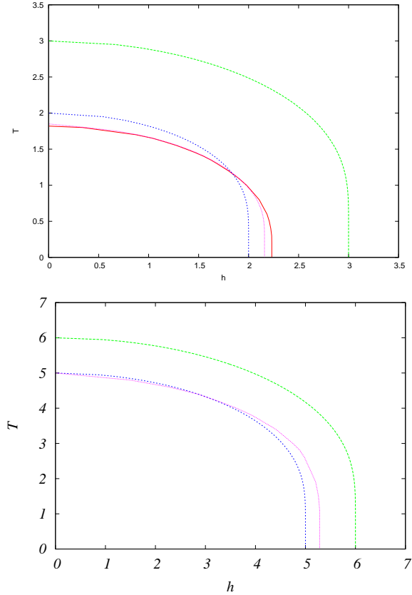
FIG. 3. Top: The phase diagram of the ferromagnet in a transverse field, on a Bethe lattice with K + 1 = 3 neighbours per spin. The plot shows the critical temperature versus transverse field, separating the low- T ferromagnetic region from the high- T paramagnetic one. The full red curve is the exact result obtained by continuous time spin trajectory population dynamics 39 . The green long-dashed curve is the naive mean field result. The blue dashed line is the result from the cavity-mean-field approximation. The dotted purple curve is the result obtained from the projected cavity mapping. Bottom: Same plots with K + 1 = 6 (without the exact result), showing that the approximation going from the projected cavity mapping to the cavity-mean-field improves at larger K , as expected, and becomes rather accurate already for this moderate value of K .
