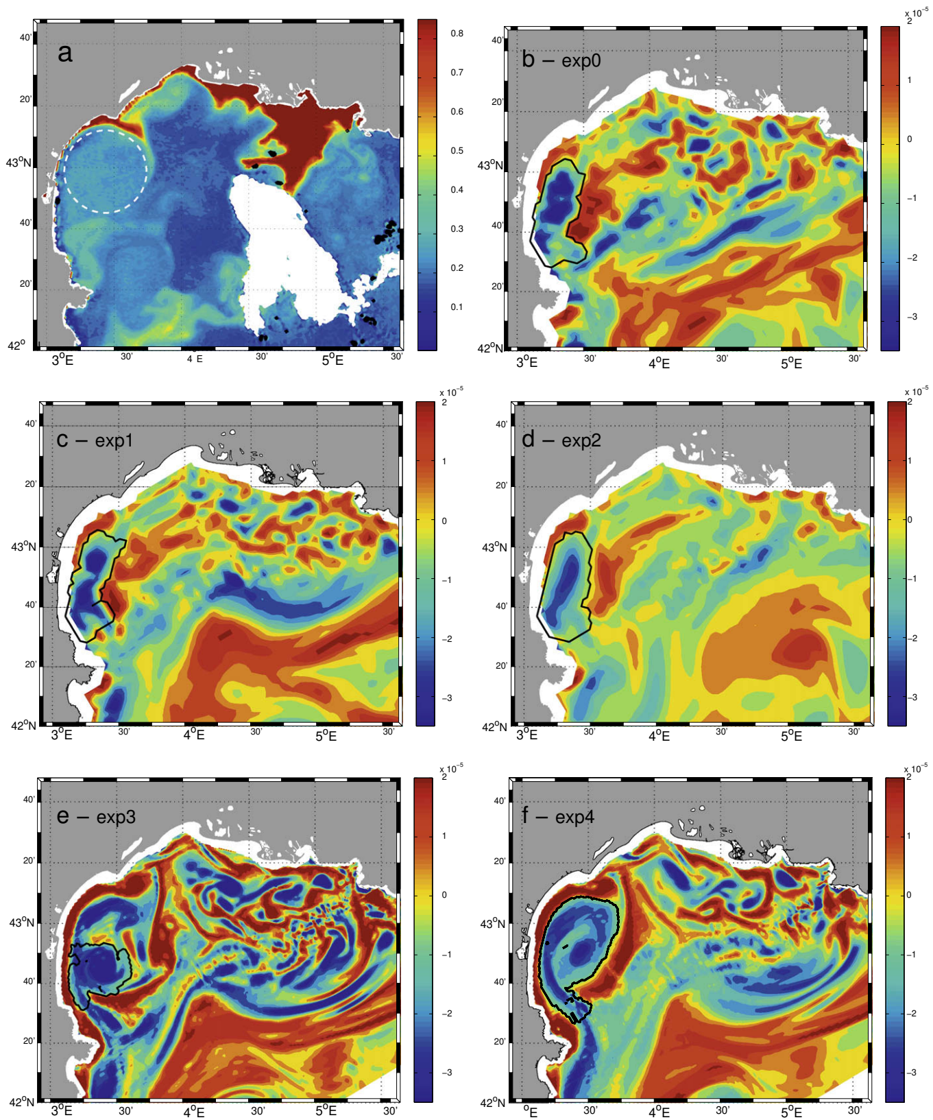
Fig. 3. Comparison of the signature of the anticyclonic eddy on a chlorophyll a [ \text{mg m}^{-3} ] map and the eddy, as identified by the wavelet analysis (contour black) of simulated relative vorticity [ \text{s}^{-1} ] on July 25, 2001. (a) SeaWiFs image processed with OC4 (courtesy E.Bosc); the dashed white circle represents the eddy area. Relative vorticity at 20-m depth from simulations (b) exp0 , (c) exp1 , (d) exp2 , (e) exp3 and (f) exp4 . See text for more explanations.
