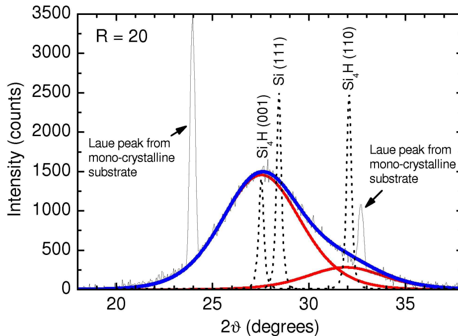
Figure 3: XRD patterns of the FSP after background correction. The peak is fitted with two Pearson VII profiles. Also shown are the XRD lines for crystalline Si and Si 4 H. 90x65mm (600 x 600 DPI)
