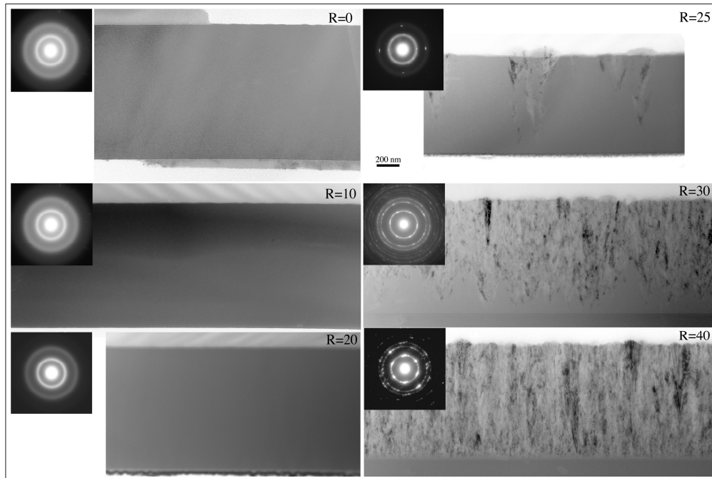
Figure 1: Bright field TEM images of a series of 1 um thick films deposited at increasing hydrogen dilution ratios from R=0 to 40.
