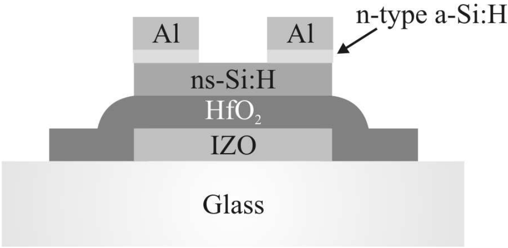
Figure 3. Schematic structure of bottom gate ns-Si:H TFTs integrating as dielectric: (c) sputtered hafnium oxide (HfO 2 )
