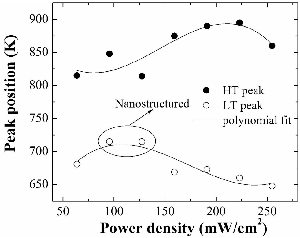
Figure 7. Evolution of LT and HT hydrogen exodiffusion peak positions as function of power density, for \text{dr}=5\% . 269x206mm (300 x 300 DPI)
