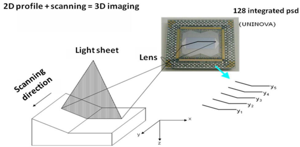
25 Figure 12. Schematic of the light line projected onto de integrated 128 psd arrays that contains the 26 information of the object to be displayed.
