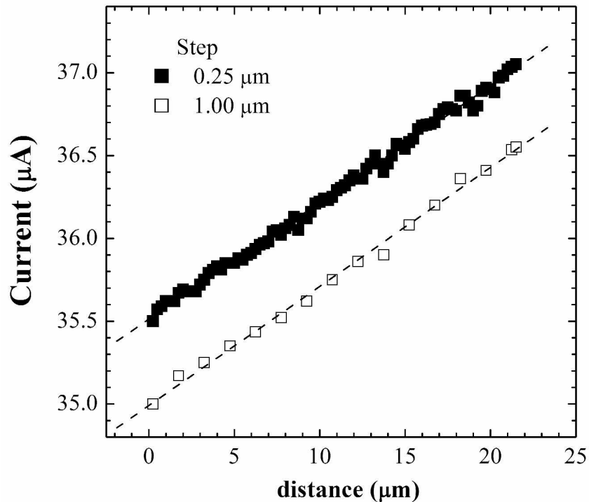
Figure 9. Spatial resolution measurements performed on a sensor with 0.25 µm and 1.00 µm steps. 266x206mm (300 x 300 DPI)
