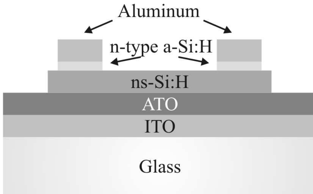
Figure 3. Schematic structure of bottom gate ns-Si:H TFTs integrating as dielectric: (a) aluminum oxide/titanium oxide multilayer (ATO) deposited by ALD;
