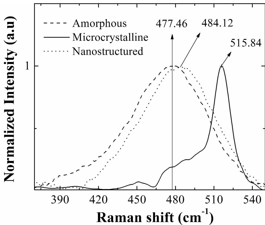
33 Figure 4. Micro-Raman spectra for the different set of silicon thin films produced. 34 269x206mm (300 x 300 DPI)
