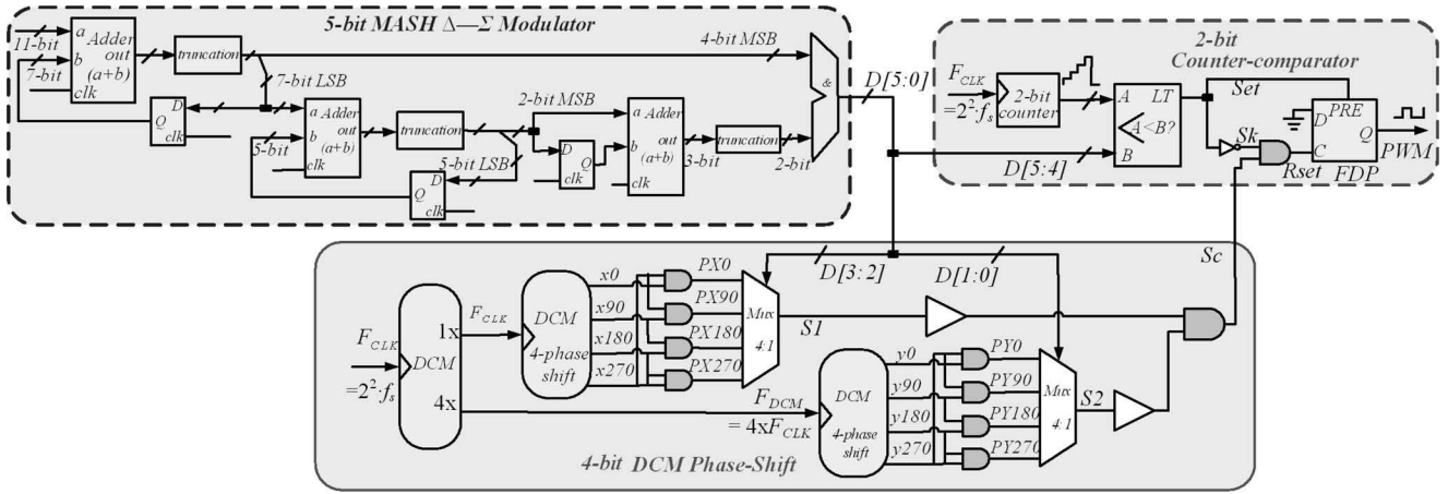
Fig. 2. Proposed 11-bit FPGA-based hybrid DPWM: 5-bit \Delta-\Sigma modulator, 4-bit segmented DCM phase-shift and 2-bit counter-comparator.
