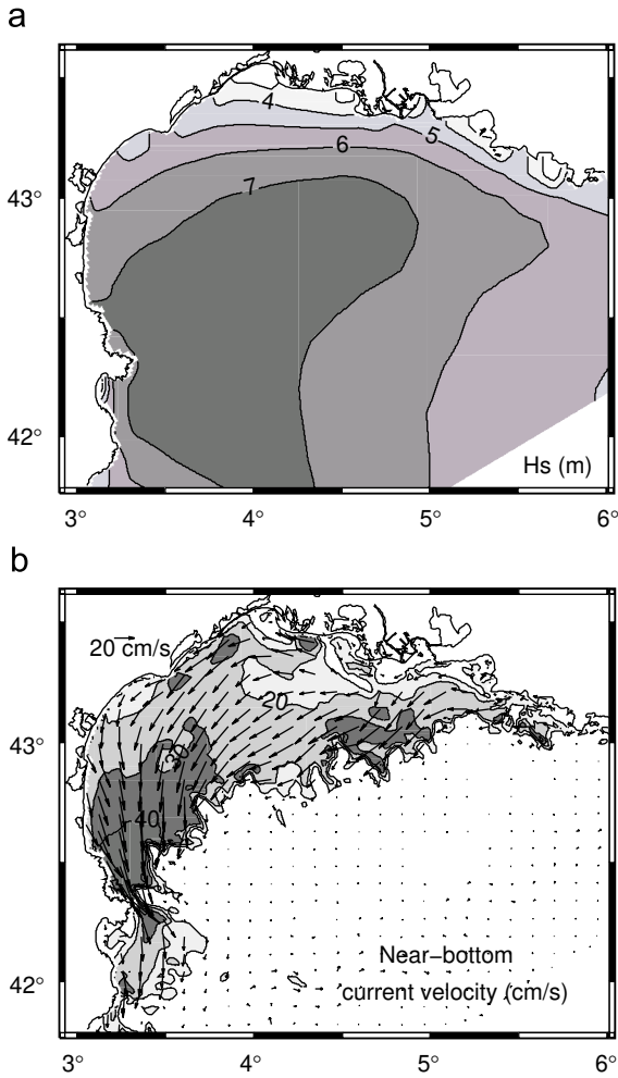
Fig. 5. (a) Significant wave height (m) and (b) near-bottom current ( \text{cm s}^{-1} ) fields simulated for the December 4, 2003 at 0:00.
