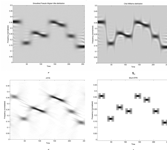
Fig. 3 - Comparison of time-frequency distributions. From left to right and top to bottom: (a) Smoothed pseudo Wigner-Ville distribution with g window width 33 and h window width 123; (b) Choi Williams distribution with smoothing parameter \sigma=3.5 ; (c) ATFR with \alpha=2 ; (d) Short ATFR of volume \alpha=25 and window width 32
