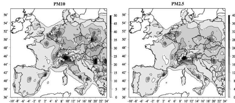
Fig. 1. Modeling results for \text{PM}_{10} and \text{PM}_{2.5} yearly mean concentrations (in \mu\text{g m}^{-3} ) in 1999.
