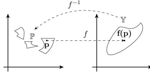
Figure 1. Illustration of our estimability approach: \mathbb{P} constitutes the reciprocal image of \mathbb{Y} = \mathbf{f}(\mathbf{p}) + \mathbb{U} .
