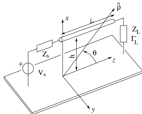
Fig. 1. The overhead line.
