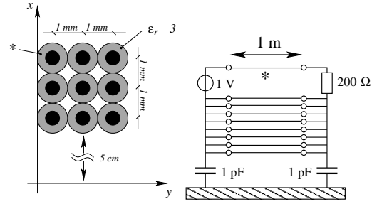
Fig. 7. The 9-wire test case for the application to an MTL. No VRs are present.
