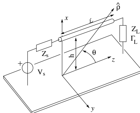
Fig. 1. The overhead line.
