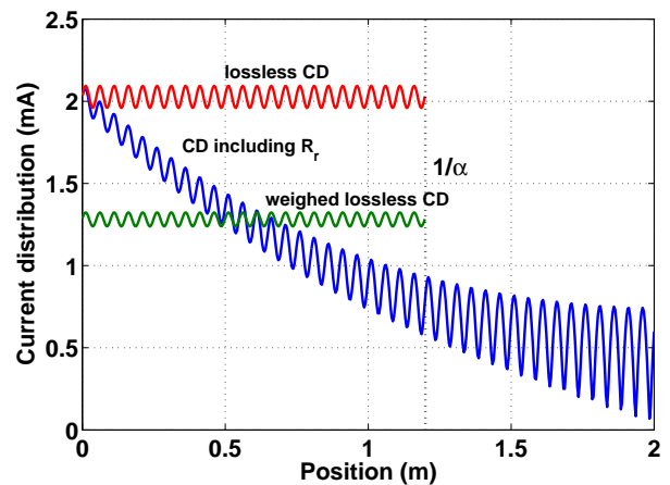
Fig. 5. An example of attenuated CD and the equivalent CDs employed by the model.
