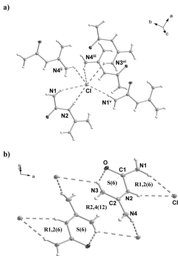
Figure 4. a) Hydrogen-bonding around the chloride anion in the crystal structure of compound 4 and b) representative hydrogen-bonding networks. Symmetry codes: (ii) 1-x, 0.5+y, 0.5-z ; (iii) 1-x, -y, -z ; (v) 1-x, -0.5+y, 0.5-z ; (vi) 1+x, y, z .
