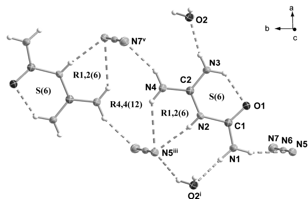
Figure 5. Hydrogen-bonding around the GU^+ cation in the crystal structure of compound 8a showing the formation of some characteristic graph-sets. Selected bond distances ( \text{\AA} ) and angles ( ^\circ ) for the N_3^- anion: N6-N5 = 1.182(1) , N6-N7 = 1.176(1) \text{ \AA} ; N5-N6-N7 = 178.7(1)^\circ .
