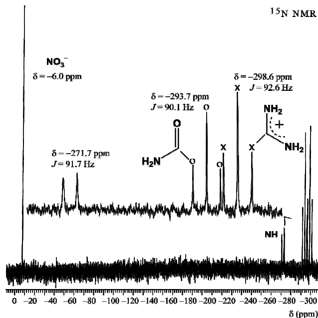
Figure 1. Coupled ^{15}\text{N} NMR of the guanylurea cation in guanylurea nitrate ( 6 ).
