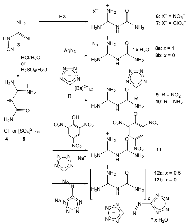
Scheme 2. Synthesis of guanlyurea salts 4–12.
