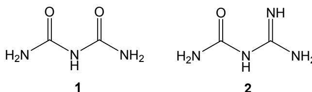
Scheme 1. Formula structures of biuret ( 1 ) and guanylurea ( 2 ).
