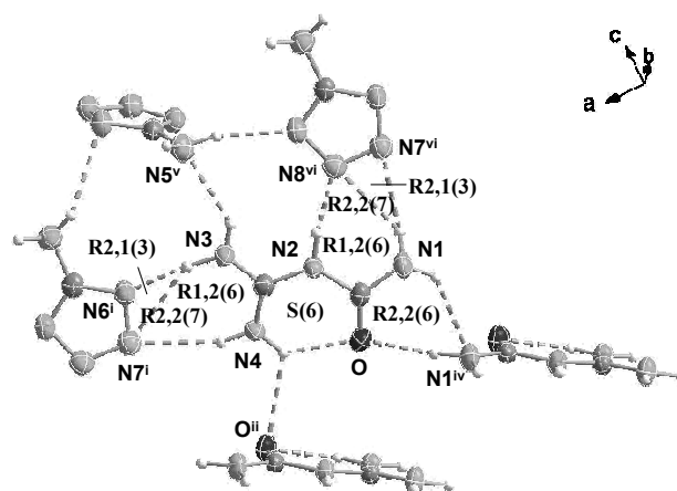
Figure 8. Hydrogen-bonding around the \text{GU}^+ cation in the crystal structure of 10 showing the formation of some characteristic graph-sets.
