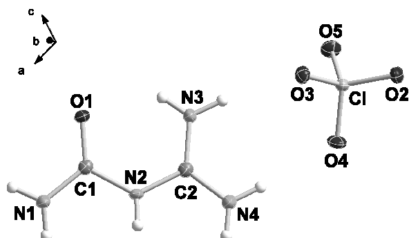
Figure 2. Asymmetric unit of 7 with the labelling scheme. Selected bond distances ( \text{\AA} ) and angles ( ^\circ ) for the \text{ClO}_4^- anion: Cl–O5 = 1.432(1) , Cl–O2 = 1.439(1) , Cl–O4 = 1.444(1) , Cl–O3 = 1.461(1) \text{\AA} ; O5–Cl–O2 = 110.3(1) , O5–Cl–O4 = 110.2(1) , O2–Cl–O4 = 110.2(1) , O5–Cl–O3 = 109.4(1) , O2–Cl–O3 = 108.9(1) , O4–Cl–O3 = 107.9(1)^\circ .
