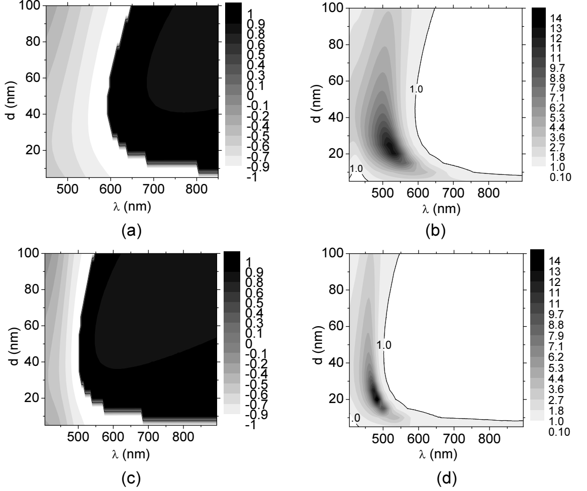
FIG. 3. (a) Phase differences normalized by \pi between the dipolar emitter and the induced dipolar moment of the nanoparticle and (b) reflection efficiency as a function of the wavelength of emission and the distance d between the emitter and the metallic surface of a 90 nm silver sphere. Figs. (c) and (d) show similar results as (a) and (b) respectively but for a 60 nm sphere.
