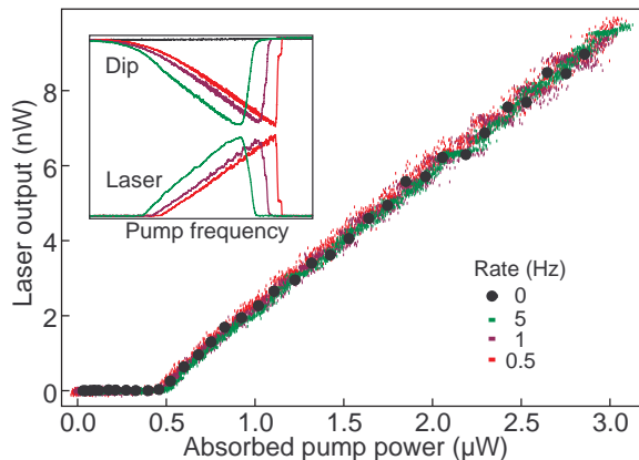
Fig. 5. (Color online) Light-light curve, for different scan speeds. Inset: corresponding transmitted pump and laser output curves.
