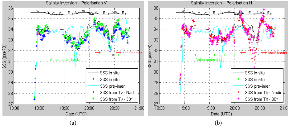
Figure 2. Sea surface salinity retrieved for the two antenna (a) in V-polarisation and (b) in H-polarisation. W, S, E represents the cardinal points and C and WW respectively Circle flights and Wing-wags movements. In situ extrapolated measurements under the plane track is plotted in black. Samples and microcat mooring are represented with a star.
