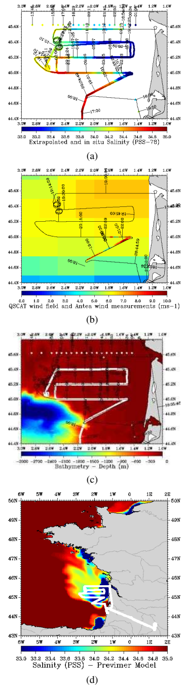
Figure 1. Sea surface conditions for the coastal flight of the 20 th May 2009 around 20 UTC. (a) Extrapolated and in situ salinity (ps-78); 1(b) QuickScat Wind Speed field (18h36) and Antea in situ wind measurements in (ms -1 ); (c) local bathymetry (meter), the plane track in black and in situ measurements in white; and (d) Sea Surface Salinity from the Previmor model taken the 20 th May 2009 at 20h UTC (Lazure & Jégou (1998)) with the plane track superimposed in white.
