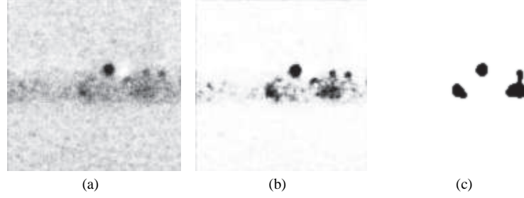
FIGURE 35. Filtered images obtained with the bistable overdamped network described by eq. (3) and (53) in the case \alpha = 1/2 . Coupling parameter: D = 0.05 . Processing times: (a) t = 4 ; (b) : t = 10 ; (c) : t = 3000 .
