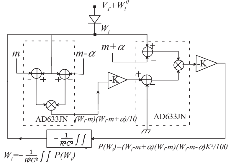
FIGURE 13. Sketch of the elementary cell of the inertial system. m and \alpha are adjusted with external DC sources whereas -K is the inverting amplifier gain obtained using TL081CN operational amplifier. The 1N4148 diode allows to introduce the initial conditions W_i^0 .
