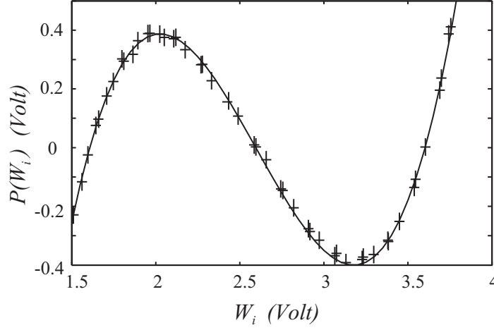
FIGURE 14. Theoretical cubic law (24) in solid line compared to the experimental characteristic plotted with crosses. Parameters: m = 2.58 \text{ V} , \alpha = 1.02 \text{ V} , K = 10 .
