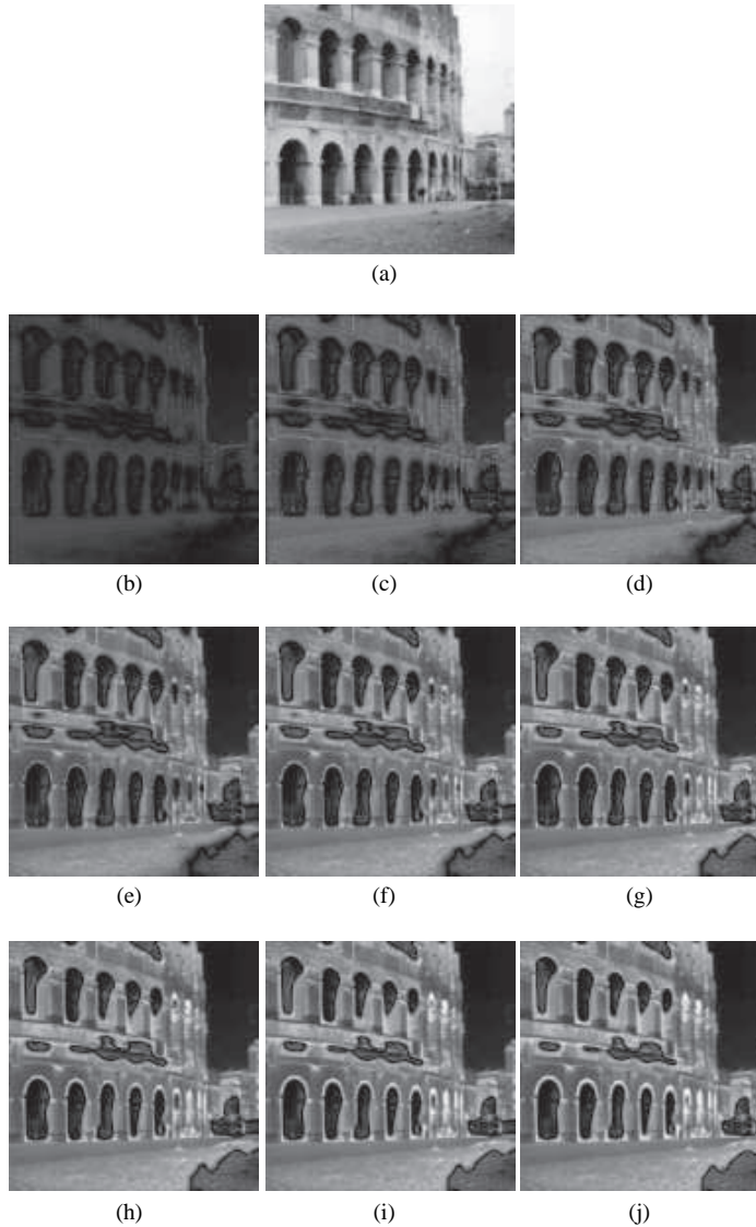
FIGURE 32. Contour enhancement of an image with 256 gray levels realized with the modified nonlinearity (54). (a) Initial image. (b), (c), (d), (e), (f), (g), (h), (i) and (j) Filtered image for the respective processing times t = 0.33, t = 0.66, t = 1, t = 1.33, t = 1.66, t = 2, t = 2.33, t = 2.66 and t = 3 .
