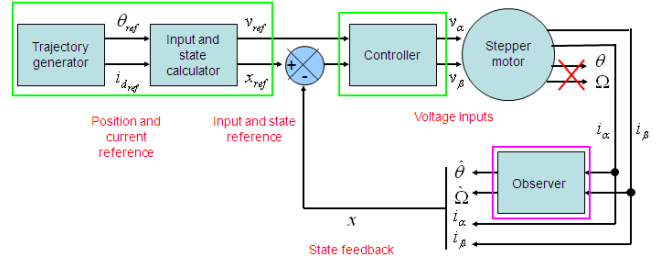
Fig. 1. Sensorless control scheme for the stepper motor
