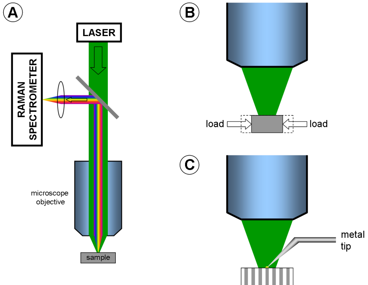
Figure 4. a) Principle of Raman spectroscopy: the laser is focused onto the sample for excitation (diffraction-limited spot \sim 1 \mu\text{m} ), then the scattered light is collected through the same objective and dispersed into a spectrum by the spectrometer. b) in-situ \mu -Raman for dynamic stress sensing: spectra are collected simultaneously during compression. c) TERS for nanoscale residual stress analysis: the metal tip localizes the excitation beyond the diffraction limit.
