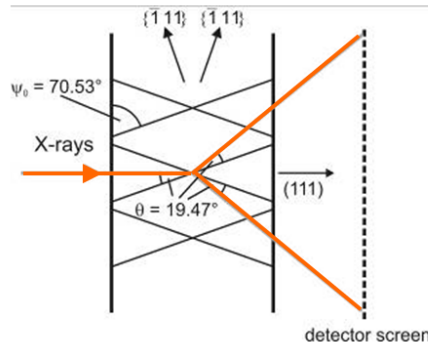
Figure 1. Comparison of diffraction geometries of the sin²ψ – technique and the sin²φ – technique. The (111) reflection is chosen for fcc metal thin films as the X-ray intensity needed to be maximized. For higher accuracy in strain higher order peaks are usually advisable.
