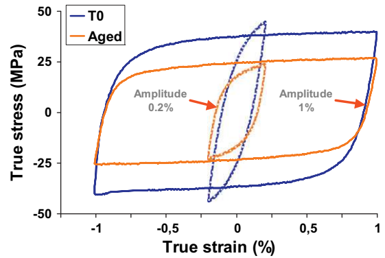
Fig. 7. Hysteresis loops at 200th cycle – strain rate: 2 \times 10^{-3} s^{-1} .
