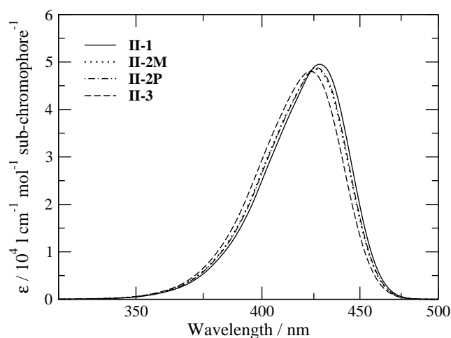
Figure 7. Calculated absorption spectra (per sub-chromophore) of the products of Series II (chloroform). Parameters in Table 3 have been used. For II-3 inhomogeneous broadening has not been accounted for and a half-width at half-maximum of 0.11 eV has been imposed.
