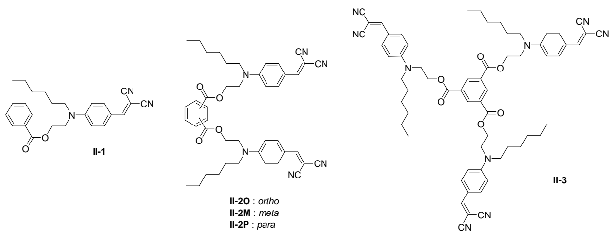
Figure 2. Compounds of Series II.
