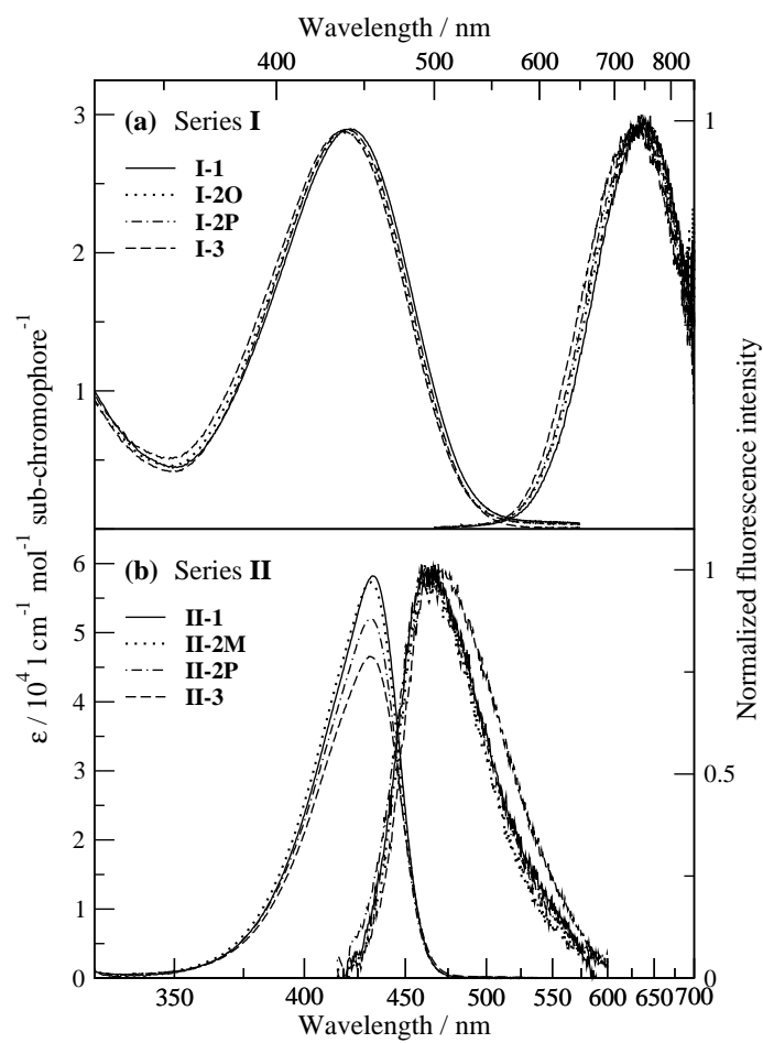
Figure 4. Absorption (per sub-chromophore) and fluorescence spectra in chloroform: (a) products of Series I; (b) products of Series II.
