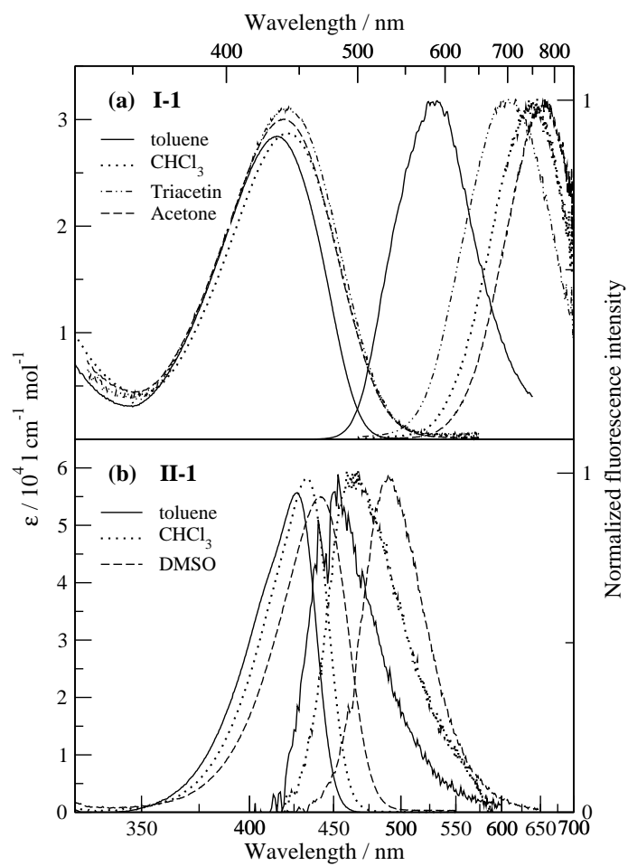
Figure 3. Absorption and fluorescence solvatochromism of the monomeric models: (a) I-1 ; (b) II-1 .
