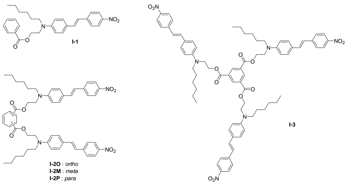
Figure 1. Compounds of Series I.
