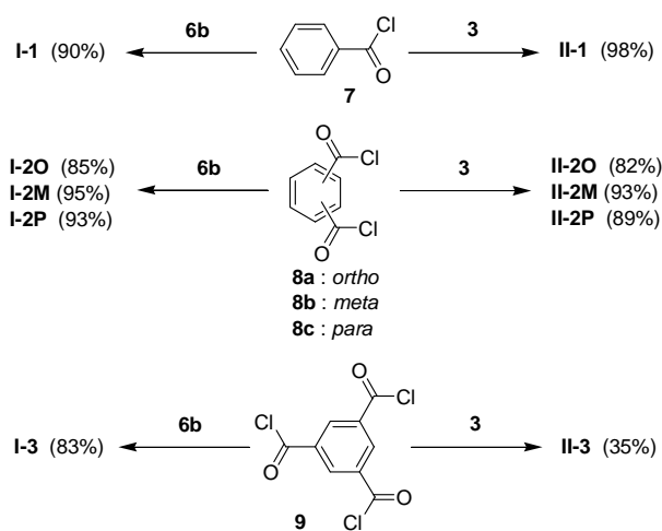
Scheme 2. Synthesis of the two series of multichromophoric assemblies. Reaction conditions: \text{NEt}_3 , \text{CH}_2\text{Cl}_2 , 20 °C, 4 h, then reflux, 1 h.
