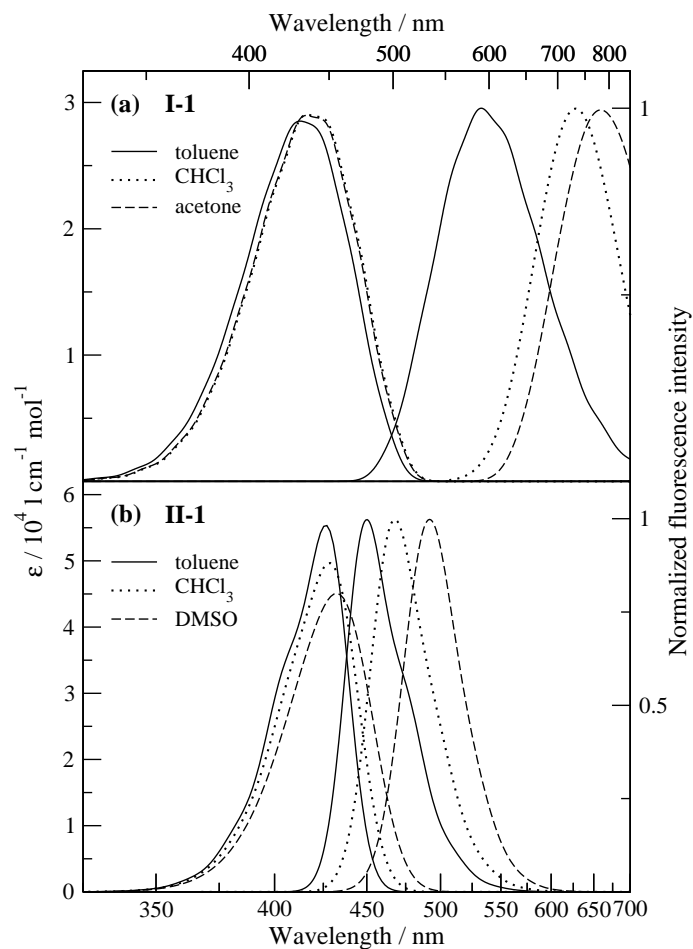
Figure 6. Calculated absorption and fluorescence solvatochromism of the monomeric models: (a) I-1 ; (b) II-1 . Parameters in Table 3 have been used.
