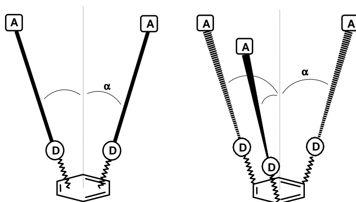
Figure 5. Schematic representation of the supramolecular structures. Spring-like lines correspond to the linkers between the central core and the active sub-chromophores. Sub-chromophores are represented by rods bearing electron-donor (D) and electron-acceptor (A) ends. For dimers and trimers C_{2v} and C_{3v} symmetries are assumed, respectively; \alpha is the angle formed by each sub-chromophore with respect to the main symmetry axis (dashed line).
