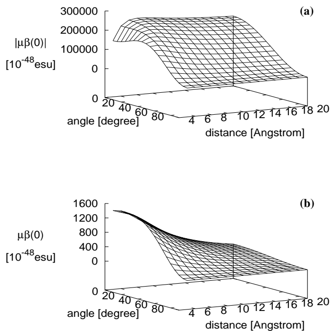
Figure 8. Angle- and distance dependence of the SHG figure of merit, calculated for a dimer ( C_{2v} symmetry) of (a) C_{16}H_{33}Q -3CNQ molecules in CHCl_3 (parameters estimated in Ref. [56] ); (b) molecules being in the cyanine limit when isolated.
