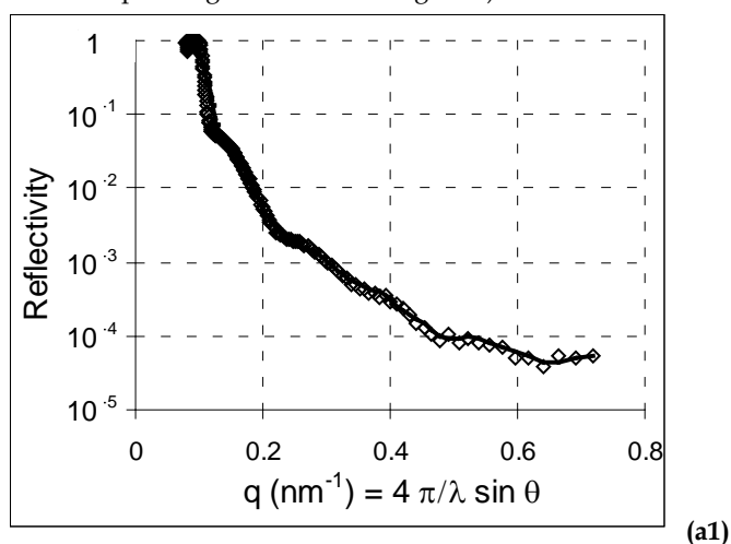
Figure 8. (ai) Neutron Reflectivity curves (raw data and fitting curves) and (bi) neutron SLD profiles deduced from the fit for PBMA 425 - b -PS 490 films doped with \gamma\text{-Fe}_2\text{O}_3\text{@PS1} nanoparticles prepared by spin-coating on silicon of 750 \mu\text{L} of a toluene solution of block copolymer (BCP) and magnetic nanoparticles (MNP) at total concentration C = 20 \text{ g/L} with increasing volume fractions \phi ( \gamma\text{-Fe}_2\text{O}_3/\gamma\text{-Fe}_2\text{O}_3\text{+BCP} ) between 0 and 0.25% (for each value, the annealing time at 150°C is also given): (a1, b1) \phi = 0.025\% (48h); (a2, b2) \phi = 0.05\% (72h); (a3, b3) \phi = 0.10\% (72h); (a4, b4) \phi = 0.15\% (72h); (a5, b5) \phi = 0.25\% (72h). A complementary study was made by keeping the volume fraction of \gamma\text{-Fe}_2\text{O}_3 at \phi = 0.025\% and varying the deposited concentration C in order to check the influence of the total film thickness on nanostructuration (Table 6 films nb. 12, 13, 14 and corresponding NR curves on Figure 9).
