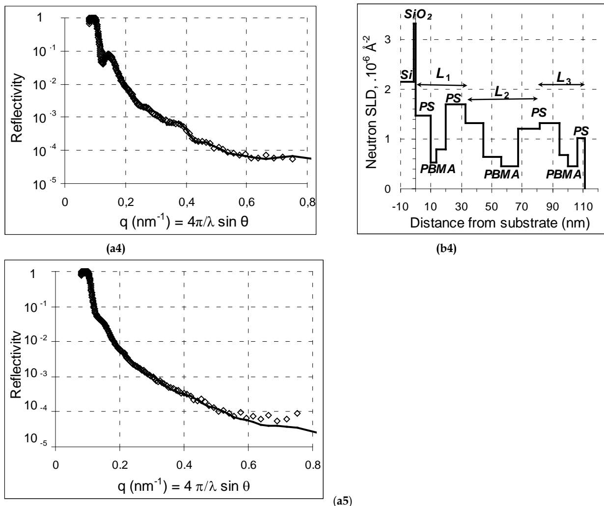
Figure 8. (ai) Neutron Reflectivity curves (raw data and fitting curves) and (bi) neutron SLD profiles deduced from the fit for PBMA 425 - b -PS 490 films doped with \gamma\text{-Fe}_2\text{O}_3\text{@PS1} nanoparticles prepared by spin-coating on silicon of 750 \mu\text{L} of a toluene solution of block copolymer (BCP) and magnetic nanoparticles (MNP) at total concentration C = 20 \text{ g/L} with increasing volume fractions \phi ( \gamma\text{-Fe}_2\text{O}_3/\gamma\text{-Fe}_2\text{O}_3\text{+BCP} ) between 0 and 0.25% (for each value, the annealing time at 150°C is also given): (a1, b1) \phi = 0.025\% (48h); (a2, b2) \phi = 0.05\% (72h); (a3, b3) \phi = 0.10\% (72h); (a4, b4) \phi = 0.15\% (72h); (a5, b5) \phi = 0.25\% (72h). A complementary study was made by keeping the volume fraction of \gamma\text{-Fe}_2\text{O}_3 at \phi = 0.025\% and varying the deposited concentration C in order to check the influence of the total film thickness on nanostructuration (Table 6 films nb. 12, 13, 14 and corresponding NR curves on Figure 9).
