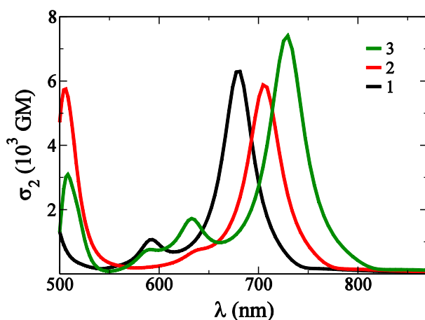
Fig. 4. Calculated TPA cross-section of chromophore 1-3.
