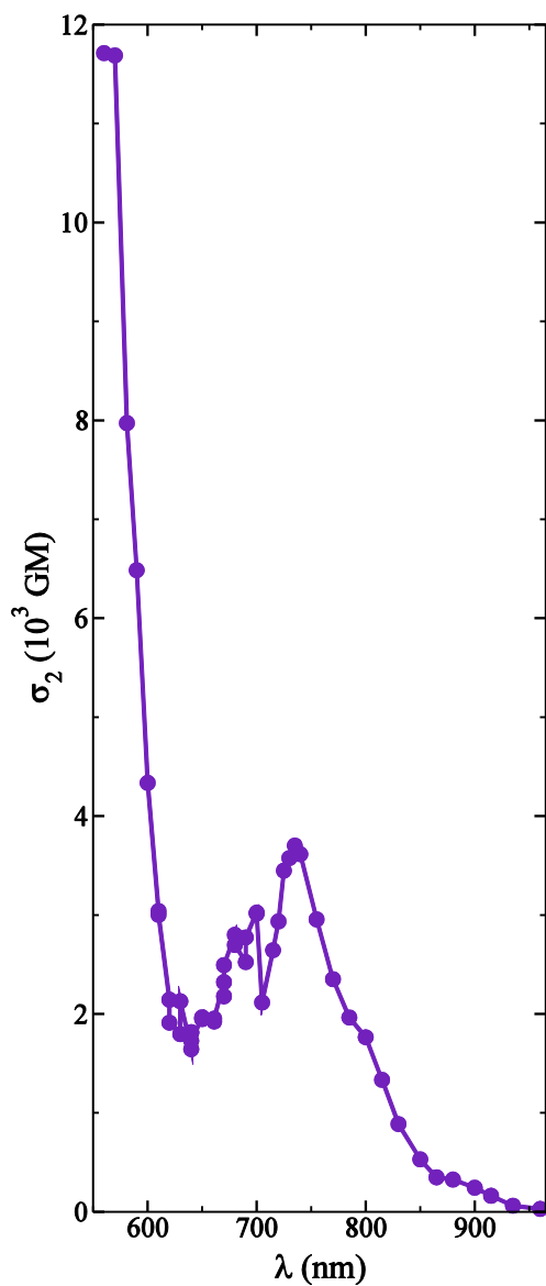
Fig. 7. Experimental TPA cross-section of the branched chromophore 4 in toluene.
