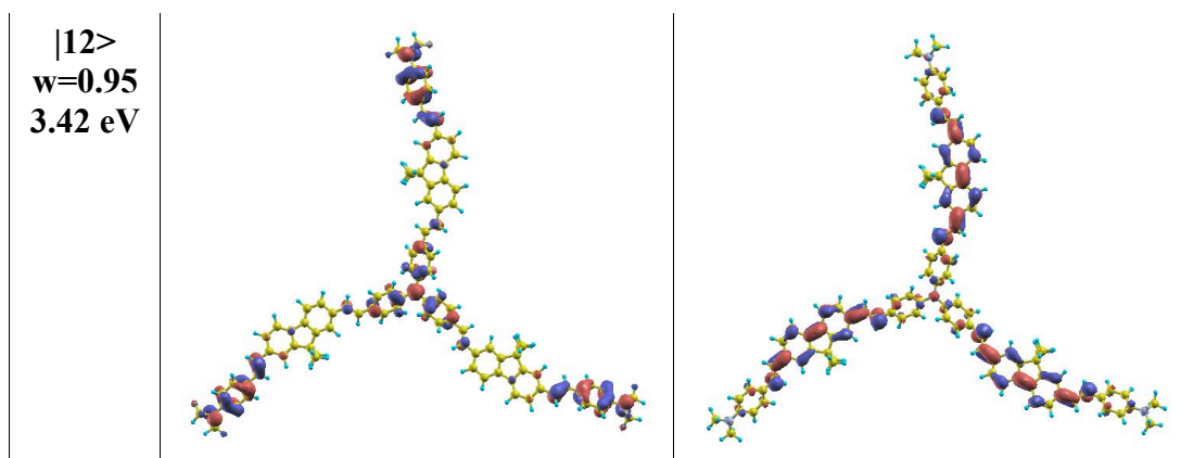
Fig. 6. Natural transition orbitals 104 of chromophore 4 : emission (top panel) absorption (all others). Right panels quote in sequence excited state number, associated eigenvalues and transition energies.
