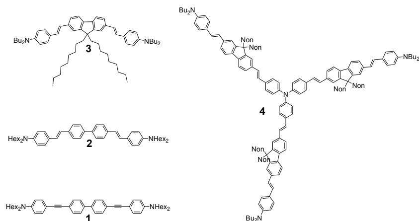
Fig. 1. Series of quadrupolar (1-3) and branched (4) chromophores.
