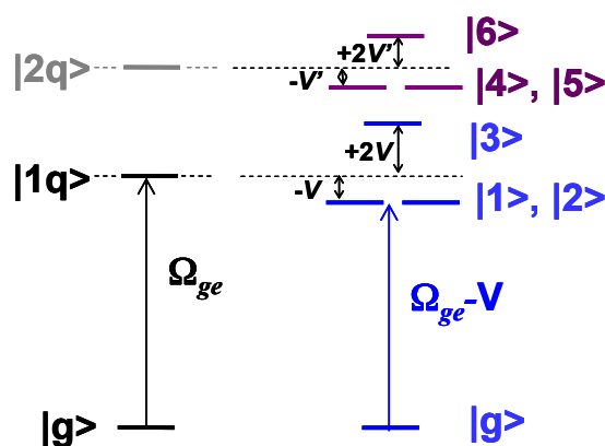
Fig. 5. Schematic electronic level diagram of the quadrupolar chromophore (left) and a molecular model of C_3 symmetry built from gathering 3 quadrupolar branches (right) within the excitonic model. |g\rangle denotes the ground state, |n\rangle the n th excited state, V ( V' ) the interbranch coupling for the quadrupolar first (second) excited state |1q\rangle ( |2q\rangle ).
