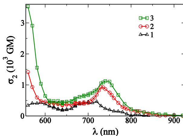
Fig. 3. Experimental TPA cross-section of quadrupolar compounds 1-3 in toluene.
