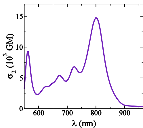
Fig. 8. Calculated TPA cross-section of the branched chromophore 4.
