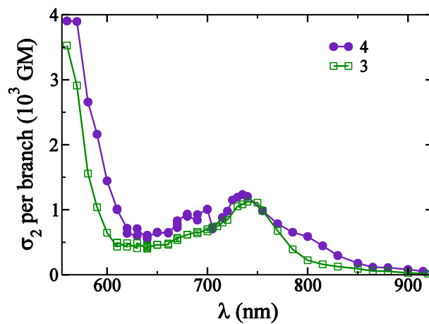
Fig. 9. Experimental TPA cross-section normalized for the number of branches of compounds 3-4 in toluene.
