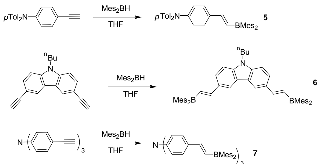
Scheme 2. Synthesis of chromophores 5-7 .
