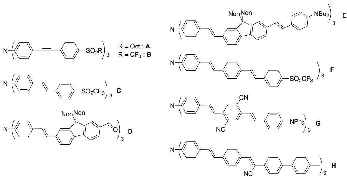
Figure 1. Molecular schemes of reference compounds for comparison to literature chromophores: A , [25b] B , [25b,35] C , [26a] D , [26a] E , [26b] F , [26a] G , [36a] H . [36b]
