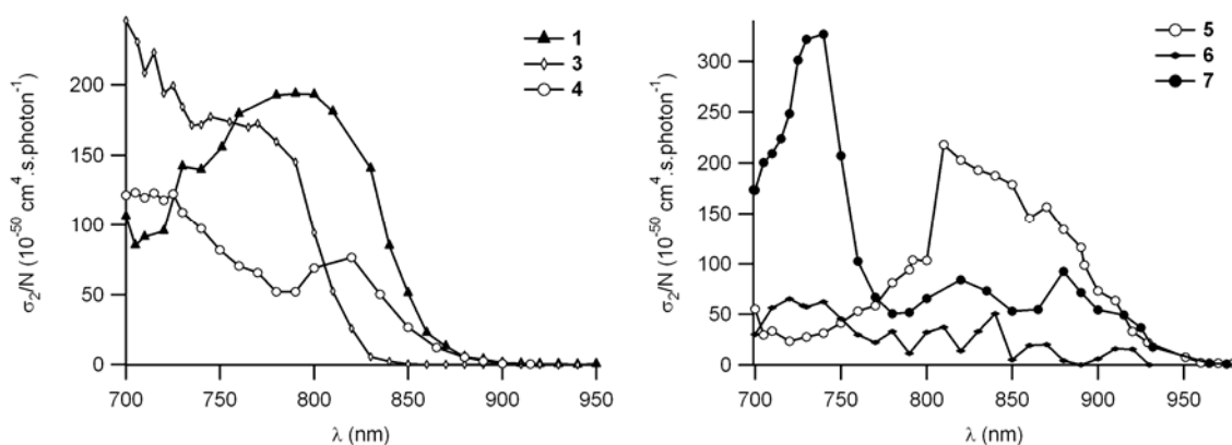
Figure 3. Comparison of the branching effect on TPA spectra normalized for the number of branches ( N ) in toluene: (left) phenylethynyl-based chromophores 1 , 3 , 4 and (right) vinylene-based compounds 5 , 6 and 7 .
