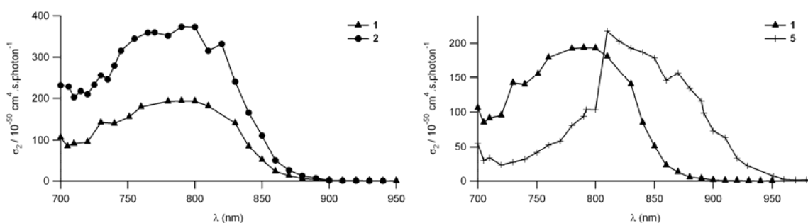
Figure 2. Comparison of TPA spectra in toluene of dipolar compounds: (left) 1 and 2 : length effect and (right) 1 and 5 : connector effect.
