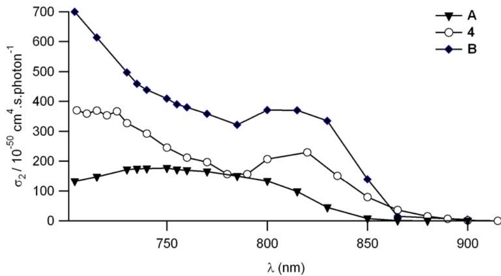
Figure 4. Comparison of TPA spectra of compound 4 with reference chromophores A [25b] and B [25b,35] in toluene: effect of the peripheral acceptor group.
