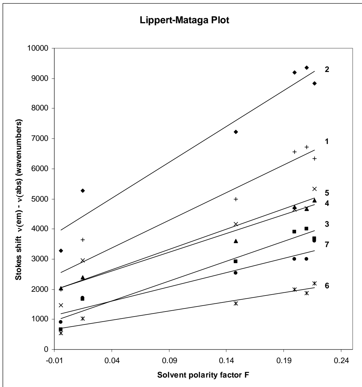
Figure S2. Lippert-Mataga plots for chromophores 1-7 .
