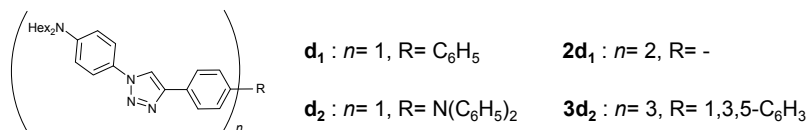
Scheme 1. Molecular structures of dipolar \mathbf{d}_1 and \mathbf{d}_2 , quadrupolar 2\mathbf{d}_1 , and three-branched 3\mathbf{d}_2 chromophores.
