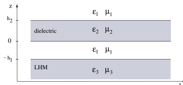
Fig. 1. Dielectric slab waveguide and the LHM interface separated by a distance h_1 and surrounded by a medium characterized by \varepsilon_1 and \mu_1 .
