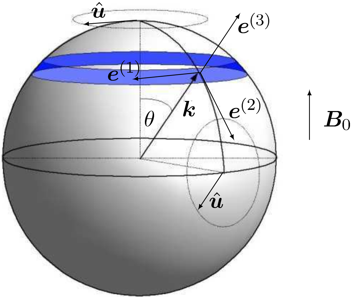
FIG. 4. Craya-Herring frame ( \mathbf{e}^{(1)}, \mathbf{e}^{(2)}, \mathbf{e}^{(3)} ) in Fourier space. Fourier modes in the blue region contribute to E(k, \theta) (eq.(7)). The polar modes ( i.e. \theta \simeq 0 ) contribute to horizontal kinetic energy, whereas equatorial modes ( i.e. \theta \simeq \pi/2 ) contribute to both vertical (along \mathbf{e}^{(2)} ) and horizontal (along \mathbf{e}^{(1)} ) kinetic energies.
