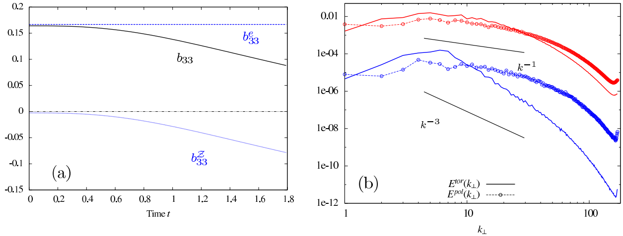
FIG. 8. (a) b_{33}(t) from a 2D-3C simulation. (b) Equatorial energy spectra E^{pol,tor}(k_\perp) . Red/top: Quasi-static 3D MHD using 512^3 Fourier modes. Blue/bottom: 2D-3C simulation using 512^2 Fourier modes (shifted down by two decades).
