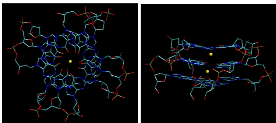
Figure 5. Top and side views of the d(\text{GGG})_4 quadruplex structure derived from molecular dynamics calculations. Sodium cations (yellow) are located in the central cavity.
