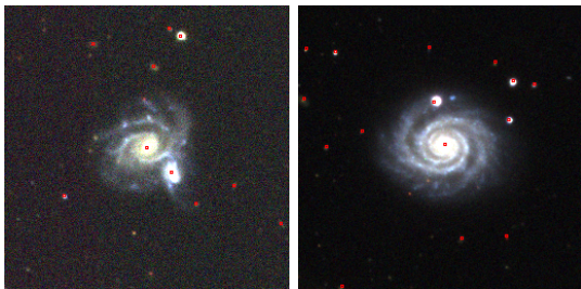
Figure 3. Source separation in two 5-band astronomical images.
