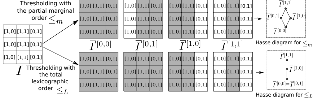
Figure 1. This example shows the Hasse diagrams of the thresholds with the marginal partial order \leq_m and a lexicographic total order \leq_L . From left to right we have: the bi-valued image, its thresholding (gray) at levels [0, 0] , [0, 1] , [1, 0] and [1, 1] , and the resulting Hasse diagrams for the two orders.
