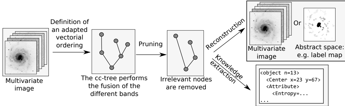
Figure 2. General framework using cc-trees
