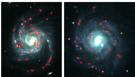
Figure 4. H II regions detection in two 5-bands astronomical images.
