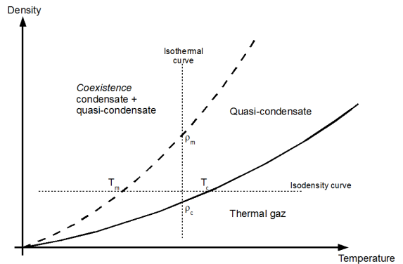
FIG. 1: Illustration of phase diagram, see (5), (7)
