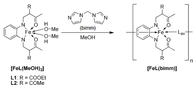
Scheme 1. General procedure for the synthesis of the 1D octahedral iron(II) coordination polymers.
