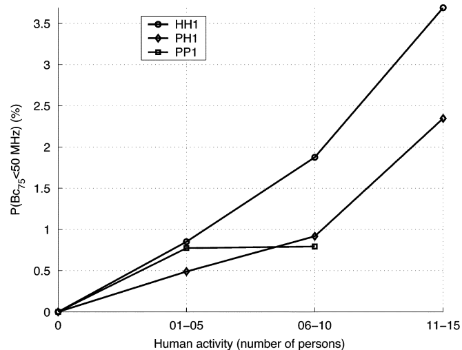
Fig. 8. Probability that the 75% coherence bandwidth is less than 50 MHz.
