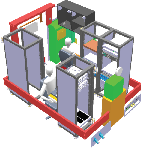
Fig. 5 Overall view of the shelter
