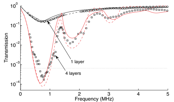
FIG. 3: Transmission of ultrasound measured through a 1-layer crystal (circles) and a 4-layer crystal (squares) with lattice constants a_x = 200 \mu\text{m} and a_z = 360 \mu\text{m} . Solid and dashed lines: predictions of the layered model and MST, respectively. Horizontal dotted line: minimum of the one-layer transmission to the fourth power.
