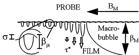
FIG. 3. Mechanism for macrobubble widening. The stress \tau^* around the macrobubble tends to swell the surrounding microbubbles. If it exceeds the value \tau_0 , these microbubbles merge and open into the macrobubble. Vertical dimensions are overmagnified.
