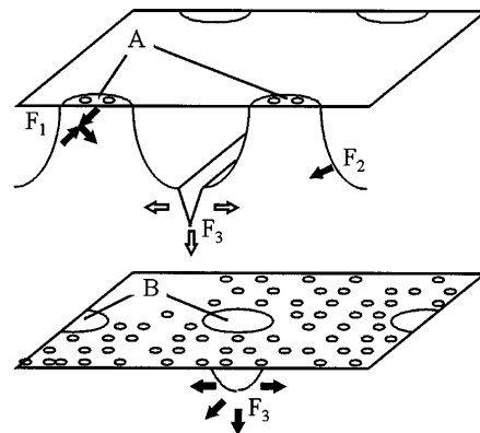
FIG. 4. Conditions for fracture initiation. Note that the amplitude of roughness has been magnified for clarity. Top: The various components of the stress tensor make it more favorable for a fracture to start along the valley lines between contact spots A (point F_3 ) than elsewhere at the interface ( F_1 or F_2 ). Bottom: Before the reverse percolation has taken place, however, there is no preferential direction for fracture initiation in the bubbles B and fracture cannot start, even though the stress intensity could be sufficient.
