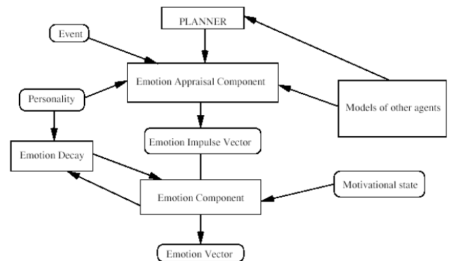
Figure 2. Architecture of ParleE
