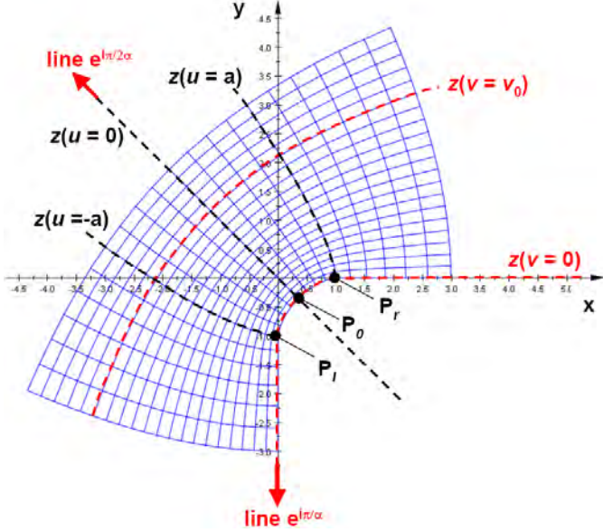
Fig. 5. z(u = \text{constant}) and z(v = \text{constant}) plotted in the z -plane for the conformal map (25)
