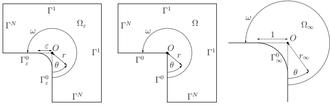
(a) Domain with rounded corner \Omega_\varepsilon . (b) Domain with a sharp corner \Omega . (c) Unbounded profile domain \Omega_\infty .
