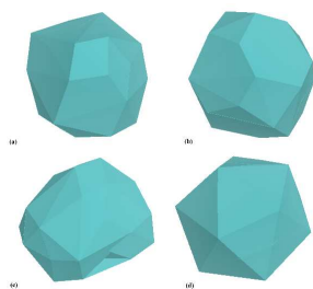
Figure 4. Comparison of optimized \text{Mo}_n cluster structures generated by RHF/AM1* optimization after sequential addition: (a) \text{Mo}_{35} , and (c) \text{Mo}_{55} , and starting at global minimum for Gupta potential: (b) \text{Mo}_{35} , and (d) \text{Mo}_{55} . Representation is polyhedral, with Mo atoms (not shown) at the vertices.
