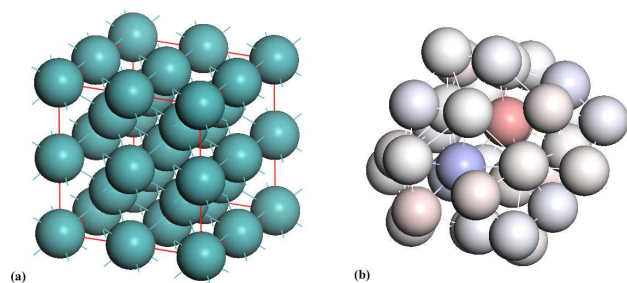
34 35 36 37 38 39 40 41 42 43 44 Figure 1. \text{Mo}_{35} nanocluster: (a) initial configuration generated from 2 \times 2 \times 2 b.c.c. supercell, and (b) the resulting structure optimized 45 at RHF/AM1* level without periodic boundaries or symmetry constraints. Mo atoms in (b) are coloured according to their Mulliken 46 charges: red -ve, blue +ve.
