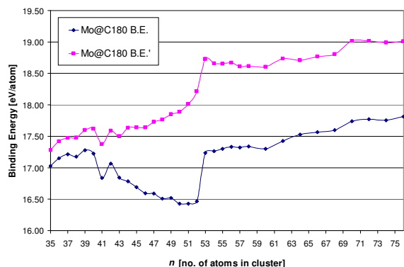
Figure 10 : Binding energies of \text{Mo}_n@C_{180} endohedral clusters, B.E._{endo} and B.E.'_{endo} , defined by Equations 2 and 3, as a function of the number of cluster atoms.
