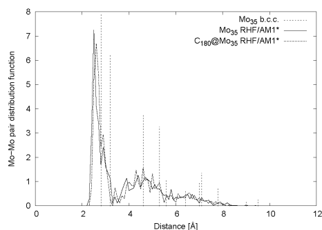
Figure 8. Mo-Mo pair distribution functions for the freestanding Mo_{35} cluster (shown in Figure 1(a)) and the Mo_{35}@C_{180} endohedral structure (shown in Figure 7(a)). The distribution for bulk b.c.c. Mo is also included for comparison.
