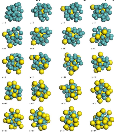
Figure 5. \text{Mo}_{(35-x)}\text{S}_x nanoclusters optimized at RHF/AM1* level. Mo atoms are shown in turquoise, and sulphur atoms in yellow.
