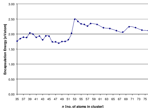
Figure 11 : Encapsulation energies of \text{Mo}_n@C_{180} endohedral clusters, E.E., defined by Equation 4, as a function of the number of cluster atoms.
