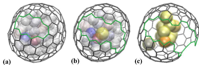
Figure 12 : RHF/AM1* optimized geometries of endohedral fullerene \text{Mo}_{(52-x)}\text{S}_x@C_{180} clusters: (a) \text{Mo}_{52}@C_{180} , (b) \text{Mo}_{51}\text{S}@C_{180} and (c) \text{Mo}_{42}\text{S}_{10}@C_{180} . In (a) and (b), Mo atoms are represented by semi-transparent spheres, coloured according to their Mulliken charges (red being negative, blue being positive) with ranges set the same for each image. In (b) and (c), sulphur atoms are highlighted by overlaying a semi-transparent yellow sphere. The fullerene defects in all three structures are highlighted in green, with full opening of fullerene cage observed in (c). As in Figure 9, bonding to Mo atoms (which terminate the dangling bonds) is not shown for clarity, and Mo atoms are also hidden in (c).
