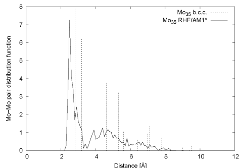
Figure 2. Mo-Mo pair distribution functions for Mo 35 structures shown in Figure 1; dashed line, Figure 1(a); solid line, Figure 1(b).
