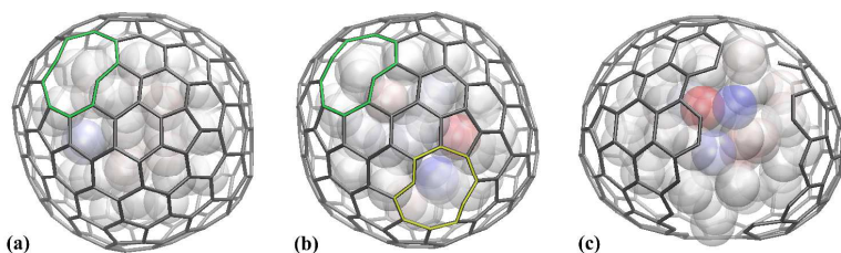
Figure 9 : RHF/AM1* optimized geometries of endohedral fullerene \text{Mo}_n clusters: (a) \text{Mo}_{44}@\text{C}_{180} , (b) \text{Mo}_{51}@\text{C}_{180} and (c) \text{Mo}_{53}@\text{C}_{180} . Mo atoms are represented by semi-transparent spheres, coloured according to their Mulliken charges (red being negative, blue being positive) with ranges set the same for each image. Fullerene defects in (a) and (b) are highlighted in green and yellow, and full opening of fullerene cage is observed in (c), with bonding to Mo atoms (which terminate the dangling bonds) not shown for clarity.
