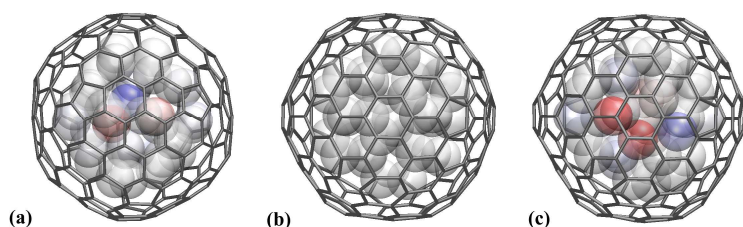
Figure 7. Endohedral fullerene Mo_n clusters: (a) Mo_{35}@C_{180} , (b) Mo_{36}@C_{180} and (c) Mo_{37}@C_{180} . Mo atoms are represented by semi-transparent spheres, coloured according to their Mulliken charges (red being negative, blue being positive) with ranges set the same for each image.
