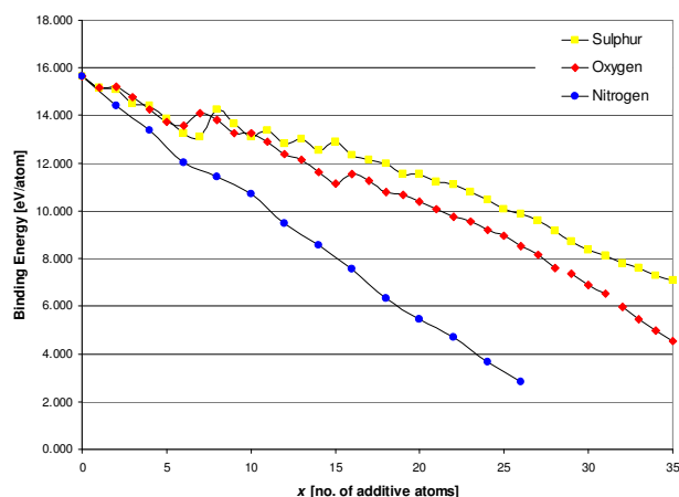
Figure 6. Behaviour of binding energy for Mo_{(35-x)}X_x clusters as a function of non-metal additive and number of additive atoms.
