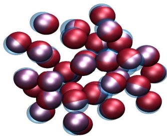
Figure 3. Aligned structures of Mo 35 nanocluster optimized with AM1* (red, solid) and B3LYP/STO-3G (blue, transparent). The r.m.s.d. between the two structures is 0.22 Å/atom (evaluated with Kabsch method).
