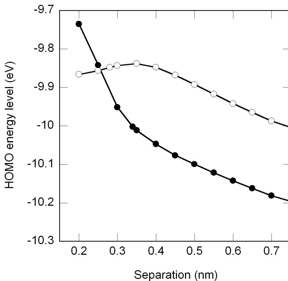
Variation of the HOMO level with intermolecular separation using the (a) VWN LDA functional (○) and (b) PW91 GGA functional (■). 105x102mm (288 x 288 DPI)
