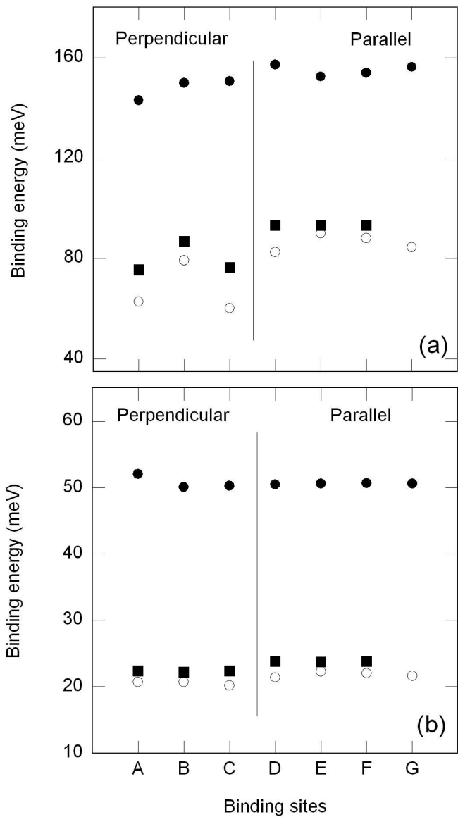
Binding energies of hydrogen physisorption on graphene and both the interior and exterior sites for using (a) VWN LDA functional and (b) PW91 GGA functional. Sites A-C correspond to the hydrogen molecular axis oriented perpendicular to the graphene or nanotube surface, whereas D-G are with the hydrogen molecular axis oriented parallel to the surface. 97x171mm (288 x 288 DPI)
