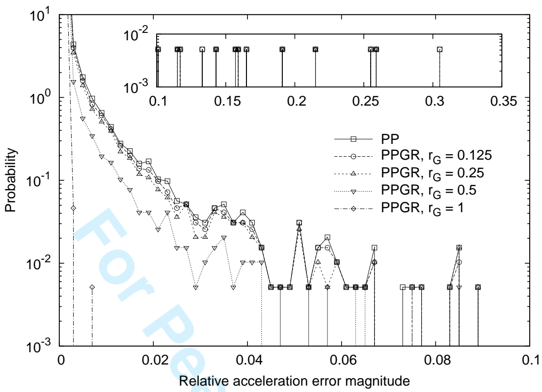
Figure 16. Relative error magnitude distribution for tetrahedral mesh, edge number 14.
