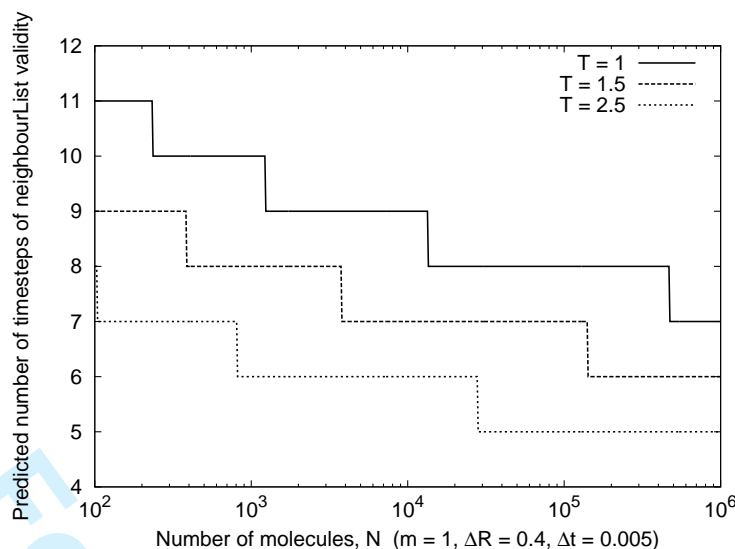
Figure A3. Variation of estimated neighbour list lifetime with typical simulation parameters for a Lennard Jones fluid [22]. T , m , \Delta R and \Delta t are in reduced MD units.
