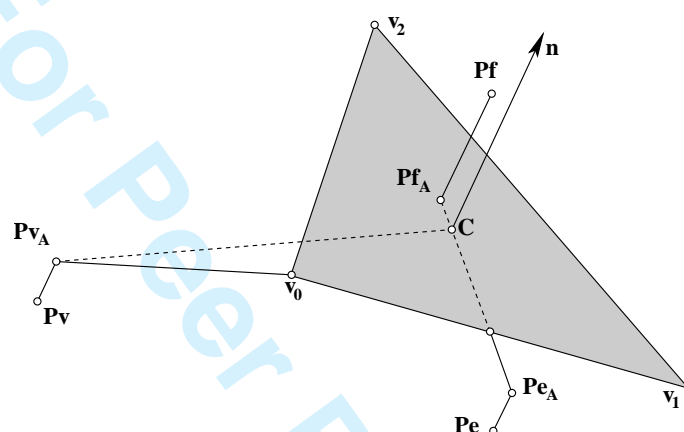
Figure 9. The three possibilities for the closest point on a face to an arbitrary point; the point is closest to a vertex, P_v , an edge, P_e , or the face itself, P_f .
