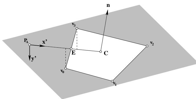
Figure 11. Defining a coordinate system local to the plane of the face to calculate intersections with face edges.
