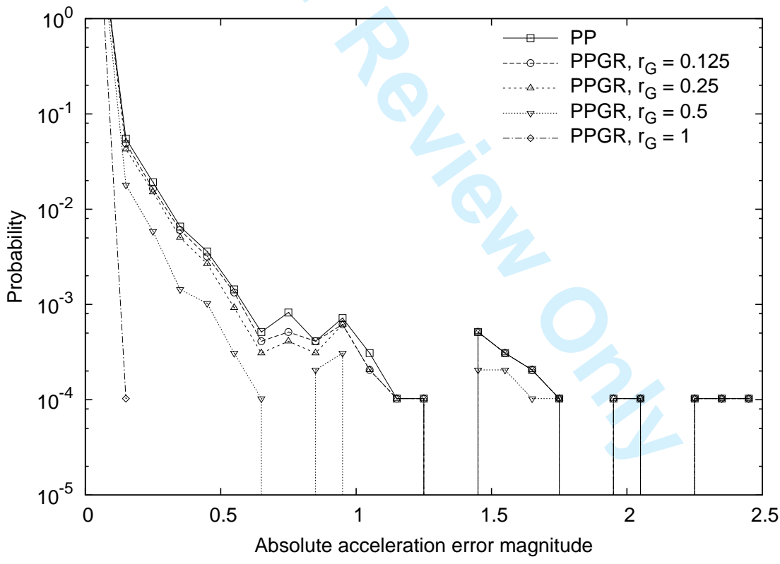
Figure 17. Absolute error magnitude distribution for tetrahedral mesh, edge number 14.
