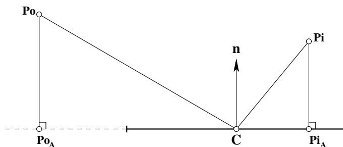
Figure 10. Projecting the point to be evaluated onto the plane defined by the face centre and normal unit vector. The projected point can either lie outside ( \mathbf{P}_{\mathbf{O}_A} ) or inside ( \mathbf{P}_{\mathbf{I}_A} ) the face.
