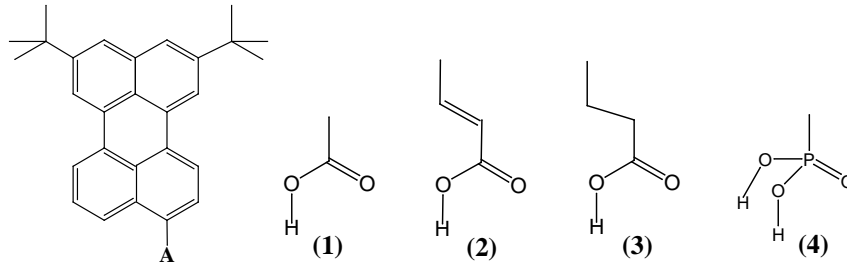
FIG. 4: Core chromophore DTB-Pe-A (di-tertiary-butyl perylene, upper panel) with bridge-anchor groups (lower panel) in position A as studied in Ref. [28]. 1 : -COOH (carboxylic acid), 2 : -(CH)=CH-COOH (acrylic acid), 3 -(CH 2 ) 2 -COOH (propionic acid), and 4 : -P(O)(OH) 2 (phosphonic acid).
